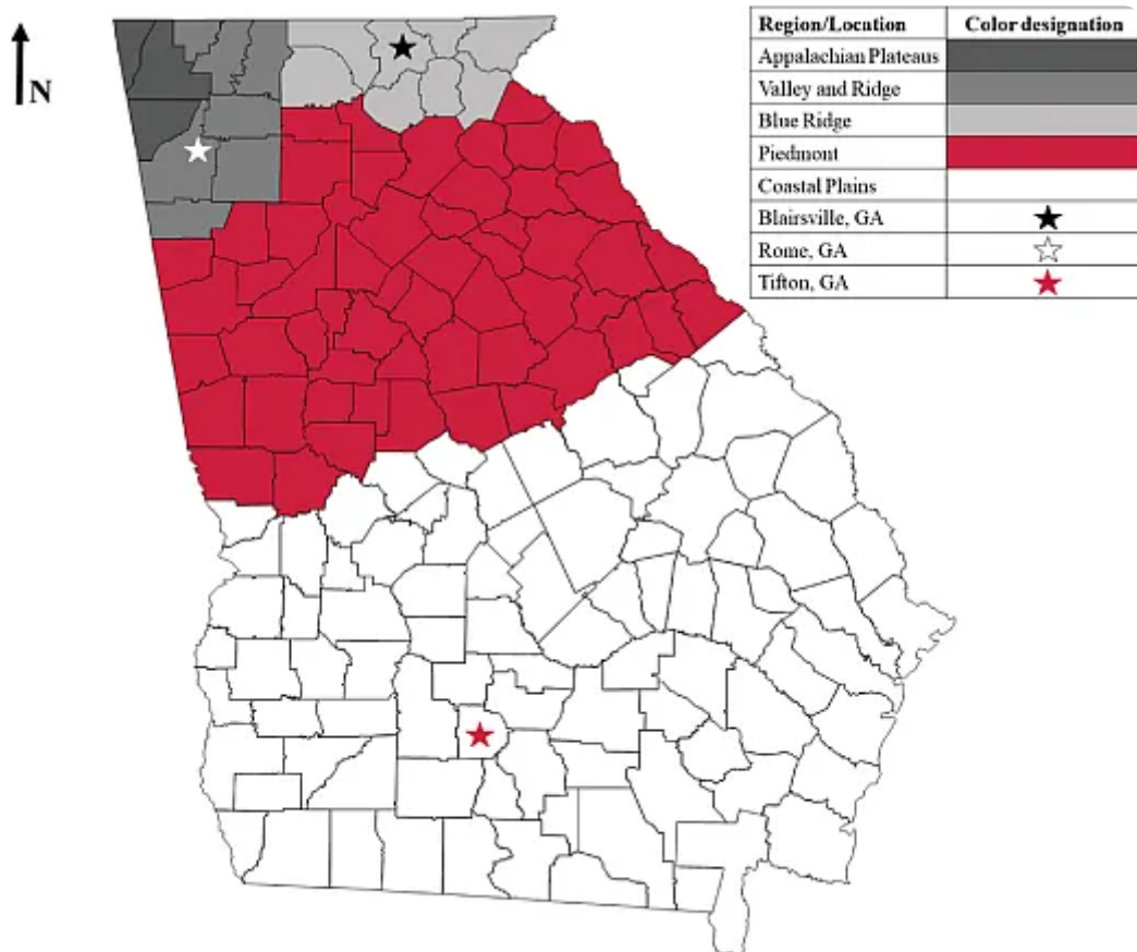
Figure 1. Georgia has five physiographic regions: Appalachian Plateaus, Valley and Ridge, Blue Ridge, Piedmont, and Coastal Plains.
