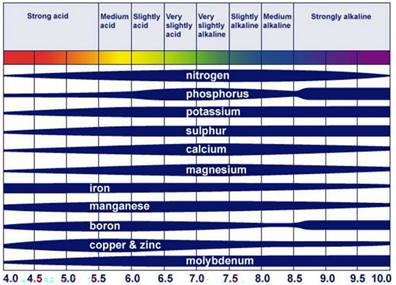
Figure 1. Effect of soil pH on the availability of nutrients. The width of the blue-colored areas indicates the relative nutrient availability to the plant/tree roots at the corresponding pH value. (Adopted: Troug, 1948).
